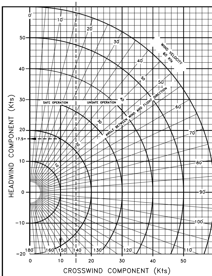
Fig.4-3.Crosswind chart
