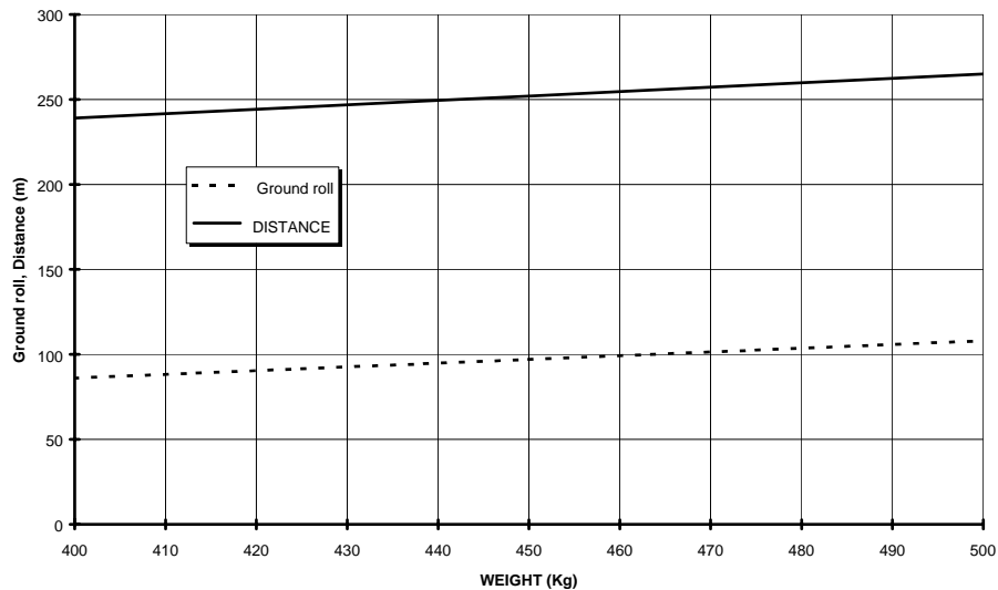
Fig. 4-7 Landing
