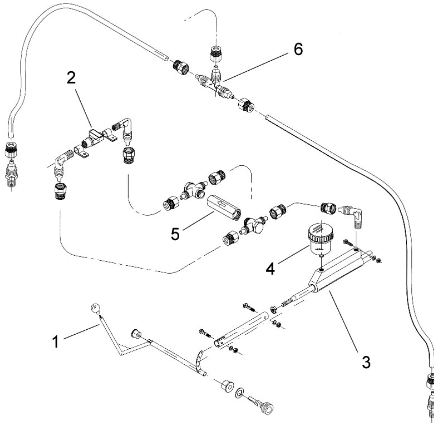
Fig. 1-7 Brake System
