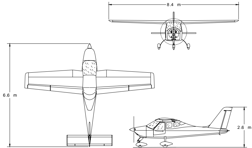
Figure 1-1 General Views
