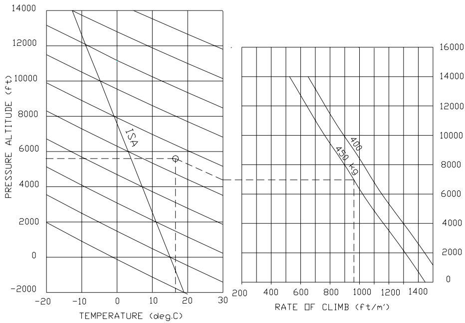
Fig. 4-5 Climb
