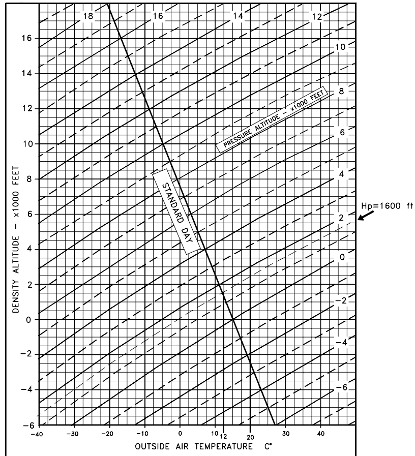
Fig.4-2. ICAO Chart
