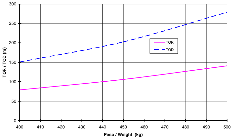
Fig. 4-4 Takeoff Performance
