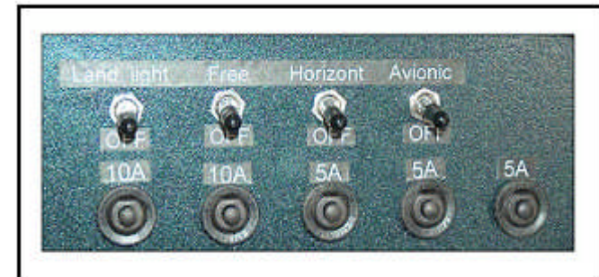
Figure 7 – Switches and fuses panel
