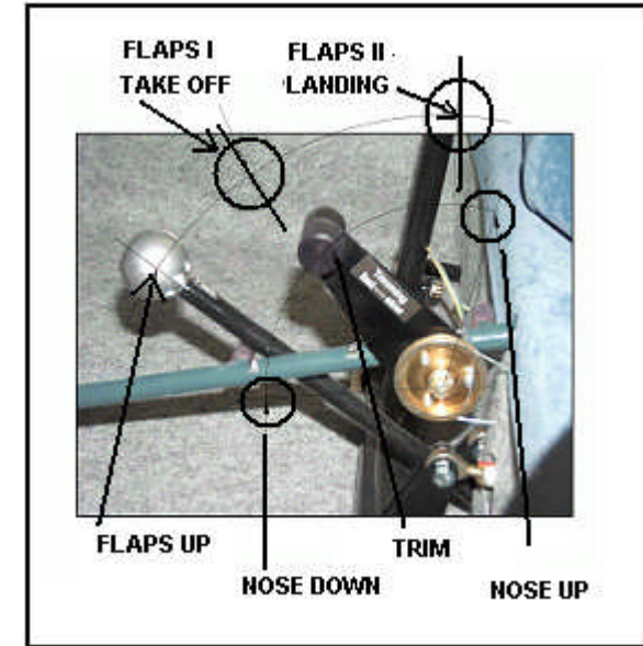
Figure 6 – Flaps and trim
